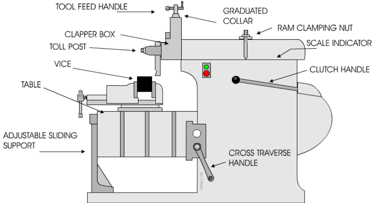
Parts of a shaping machine
