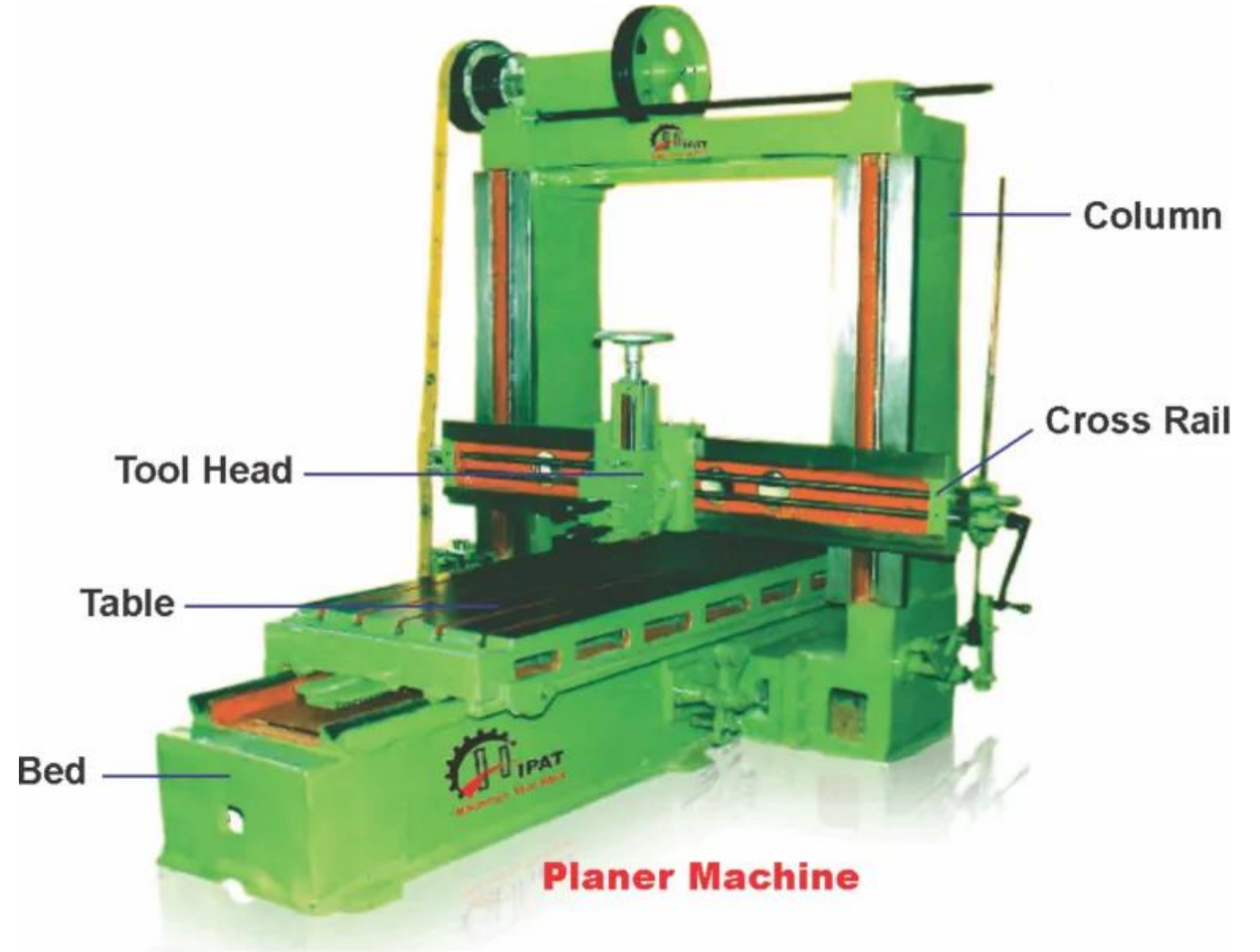
Parts of a planing machine
