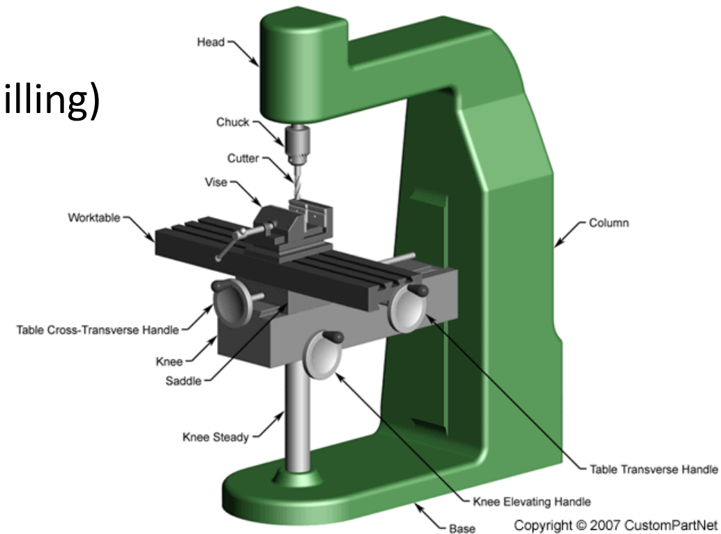
Vertical milling machine
